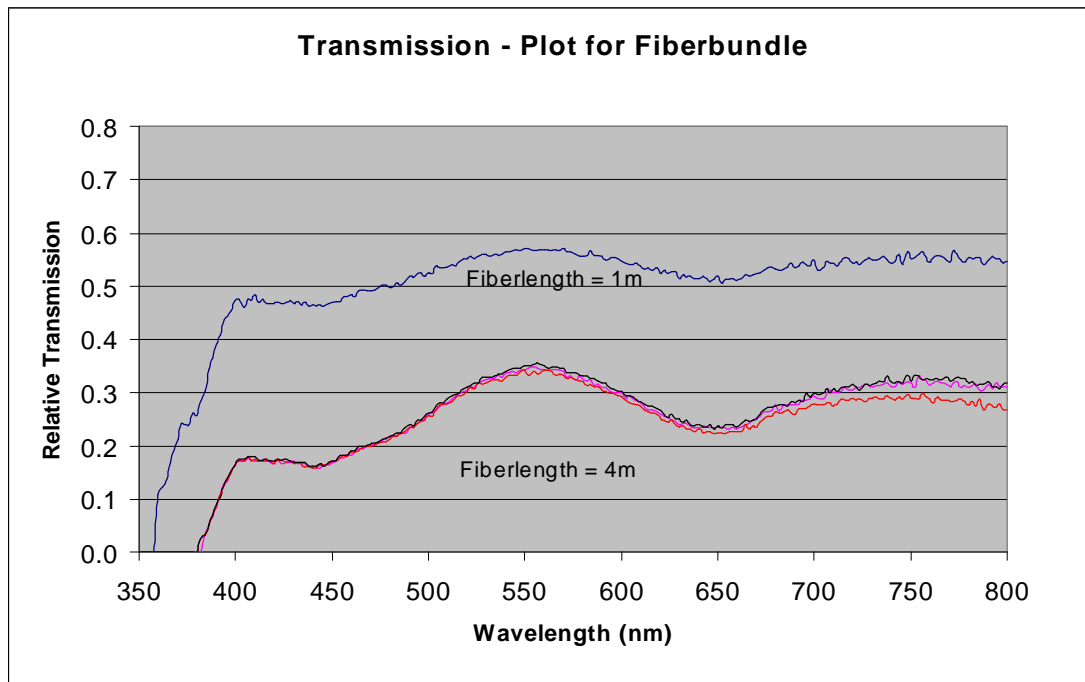
Figure 17. Fiber Bundle transmission curve (l = 1m,4m; d = 3 mm; NA = 0.55)
