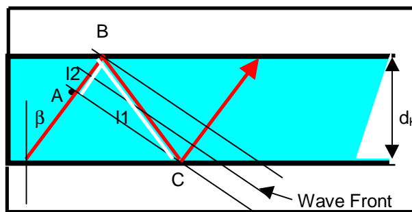
Fig. 6. Propagation within the light guide should produce the same amplitude at point A and point C (i.e. a maximum). The thickness of the propagating film is d_k .
