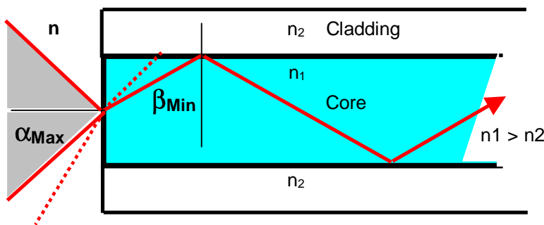
Fig. 3: Light transmission Medium n_1 with total reflection of the transmitted ray; The light guide has a cladding material n_2 ; n \dots Index of refraction for the coupling medium (usually air; n = 1 )
